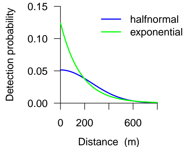
Fig. 1. (a) Hypothetical Poisson distribution of range centres near an array of detectors. Each dot represents one individual. SECR estimates the density of this distribution. (b) Alternative detection functions. The halfnormal is defined by g(d) = g_0 \exp\left(\frac{-d^2}{2\sigma^2}\right) and the exponential by g(d) = g_0 \exp\left(-\frac{d}{\sigma}\right) . See ?detectfn for more.
