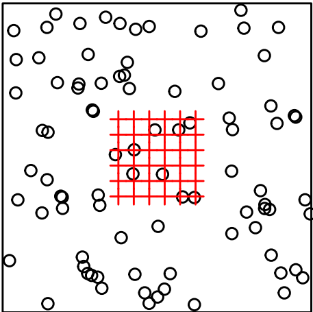
Fig. 1. (a) Hypothetical Poisson distribution of range centres near an array of detectors. Each dot represents one individual. SECR estimates the density of this distribution. (b) Alternative detection functions. The halfnormal is defined by g(d) = g_0 \exp\left(\frac{-d^2}{2\sigma^2}\right) and the exponential by g(d) = g_0 \exp\left(-\frac{d}{\sigma}\right) . See ?detectfn for more.
